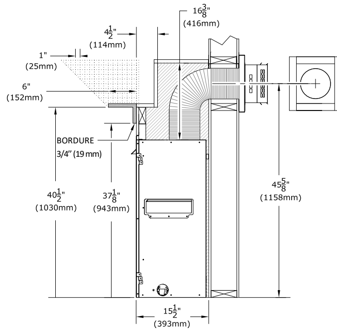
Figure 4.1 - Projections du manteau
